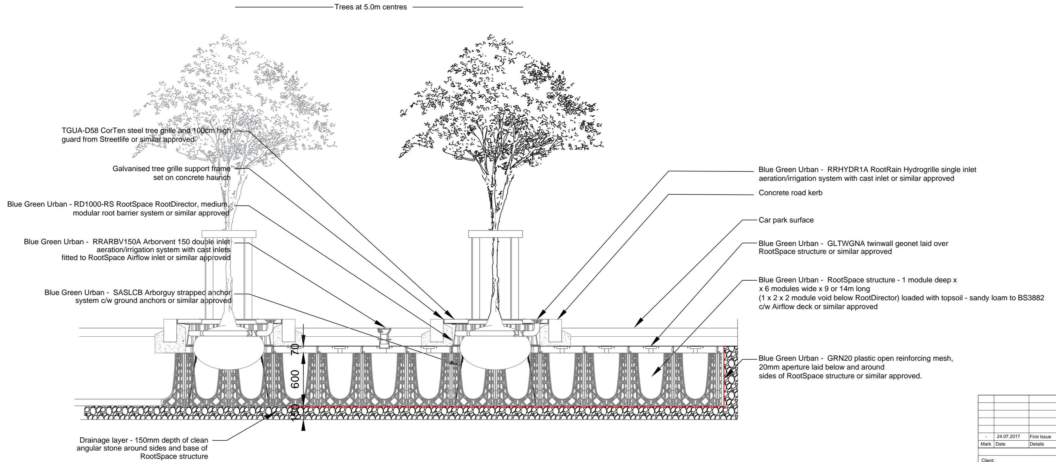
SECTION TREE TRENCH DETAIL - TREE PLANTING WITHIN CAR PARK (Scale 1:25)
