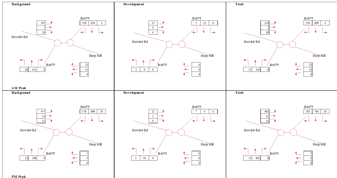
Figure 6: Priors Rd / Harp Hill / Hewlett Road Double Mini-roundabout Traffic Flows
